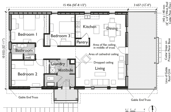
FLOOR PLAN OF TR'ONDËK HWËCH'IN NORTHERN SUSTAINABLE HOUSE
